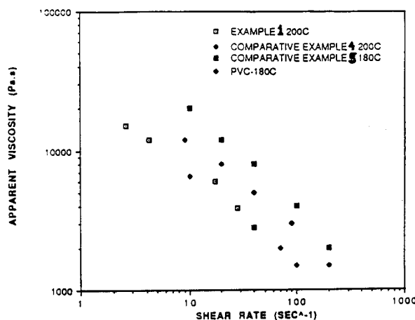
FIGURE 1: VISCOSITY VERSUS SHEAR RATE FOR RESIN COMPOSITIONS
