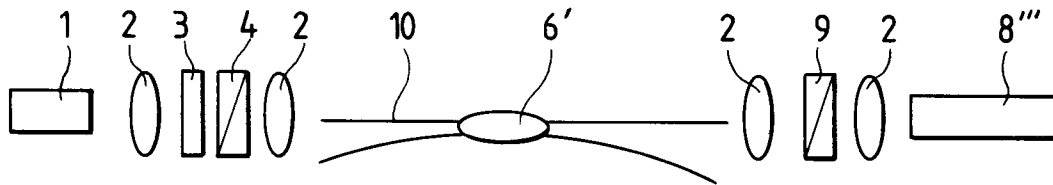
FIG. 2 PRIOR ART
