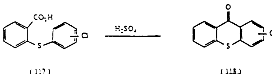
Scheme 54
