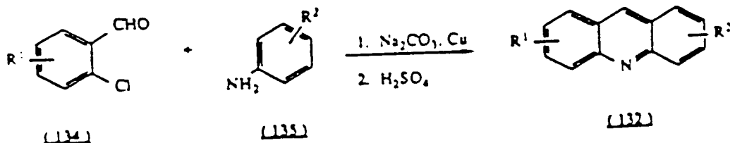
Scheme 62
