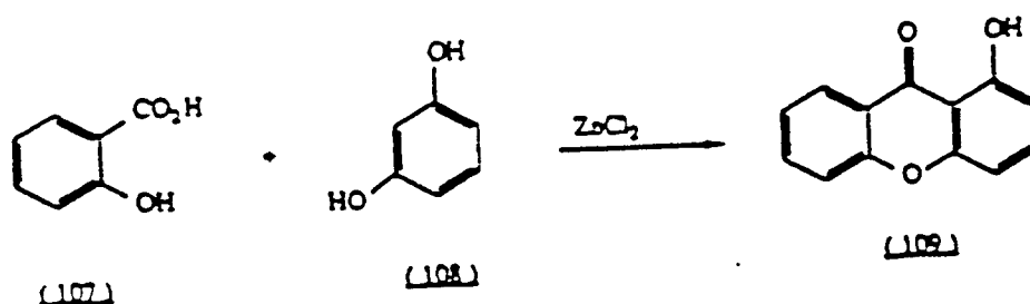
Scheme 50
