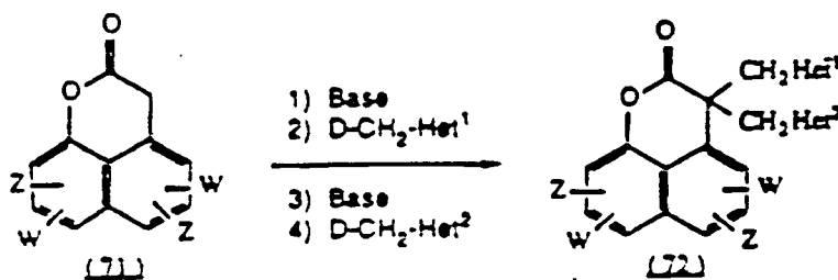
Scheme 31
