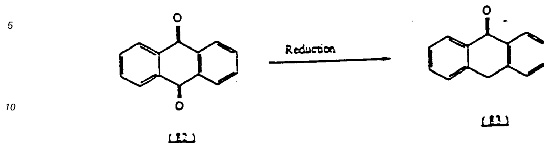
Scheme 36
