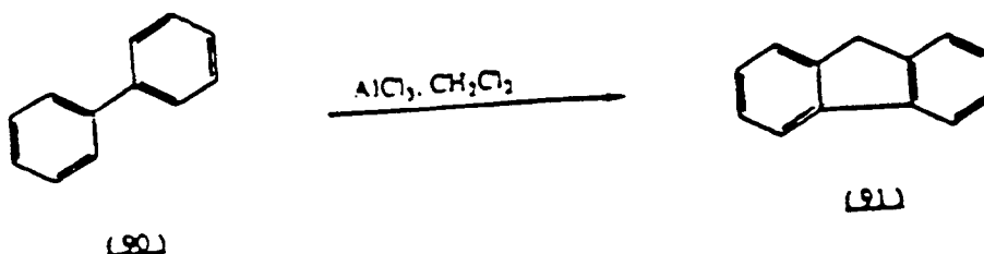
Scheme 40
