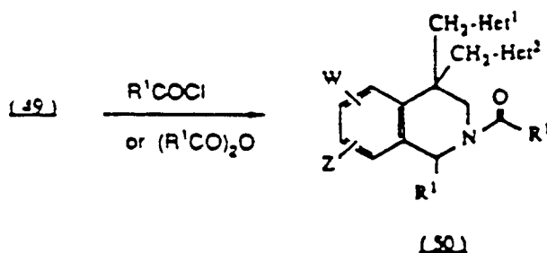
Scheme 20
