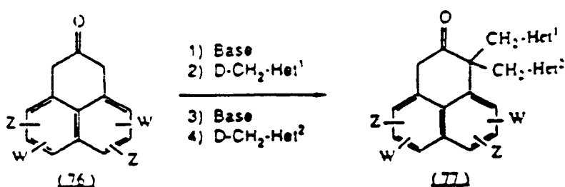
Scheme 33
