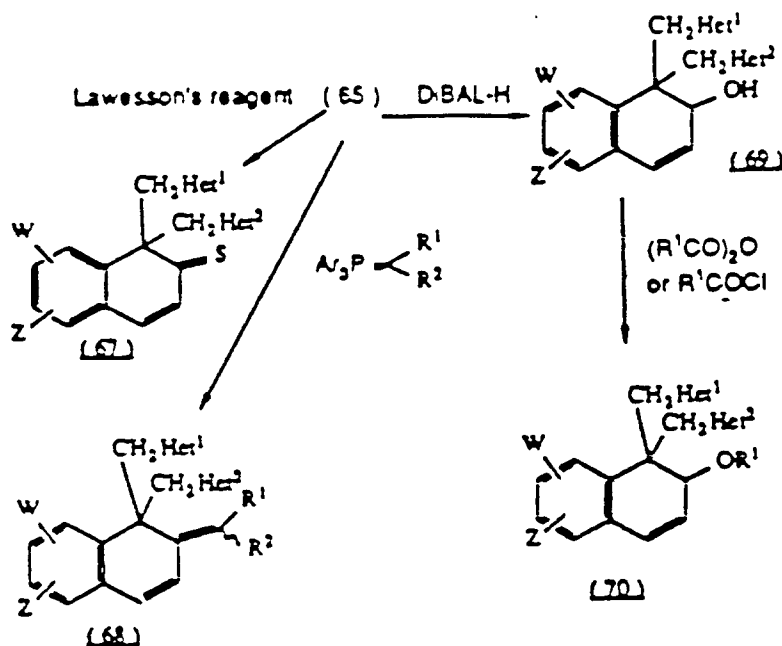
Scheme 30
