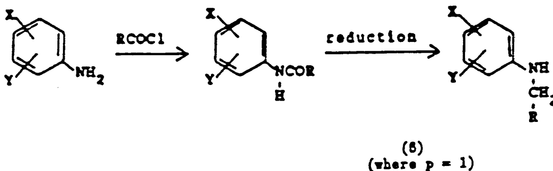
Scheme 4
