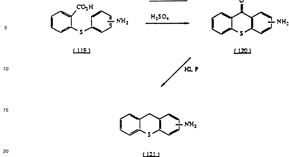
Scheme 55
