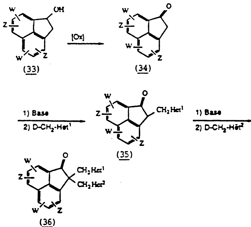
Scheme 13
