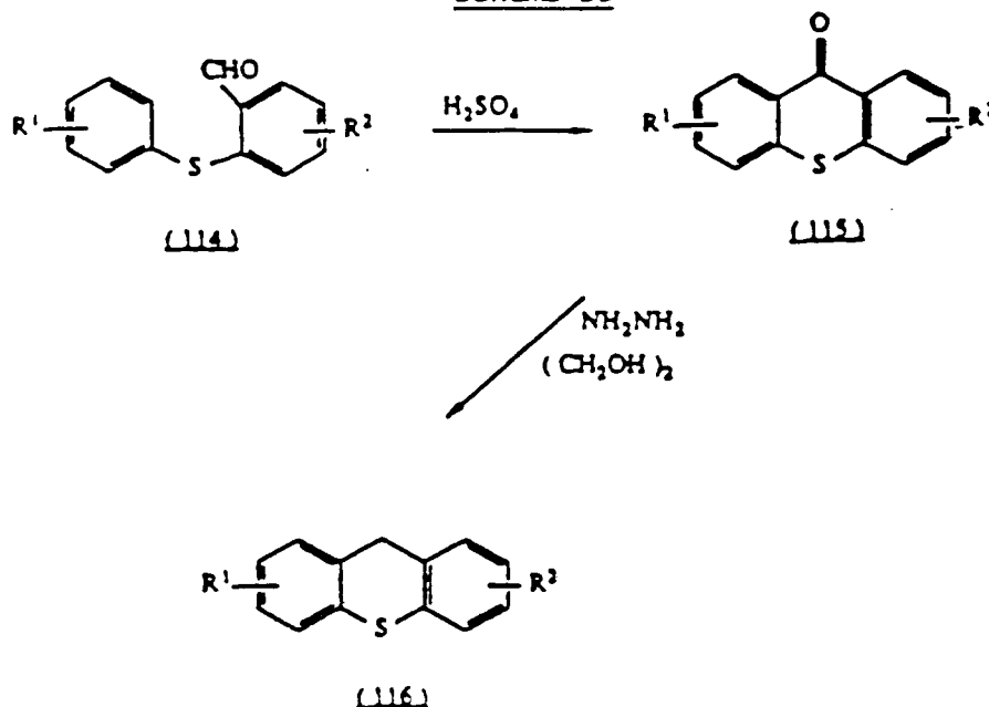
Scheme 53
