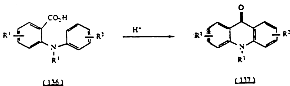
Scheme 63
