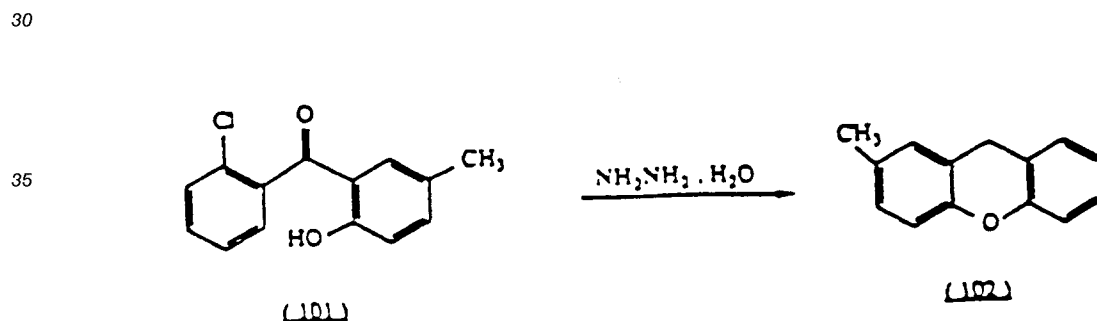
Scheme 46
