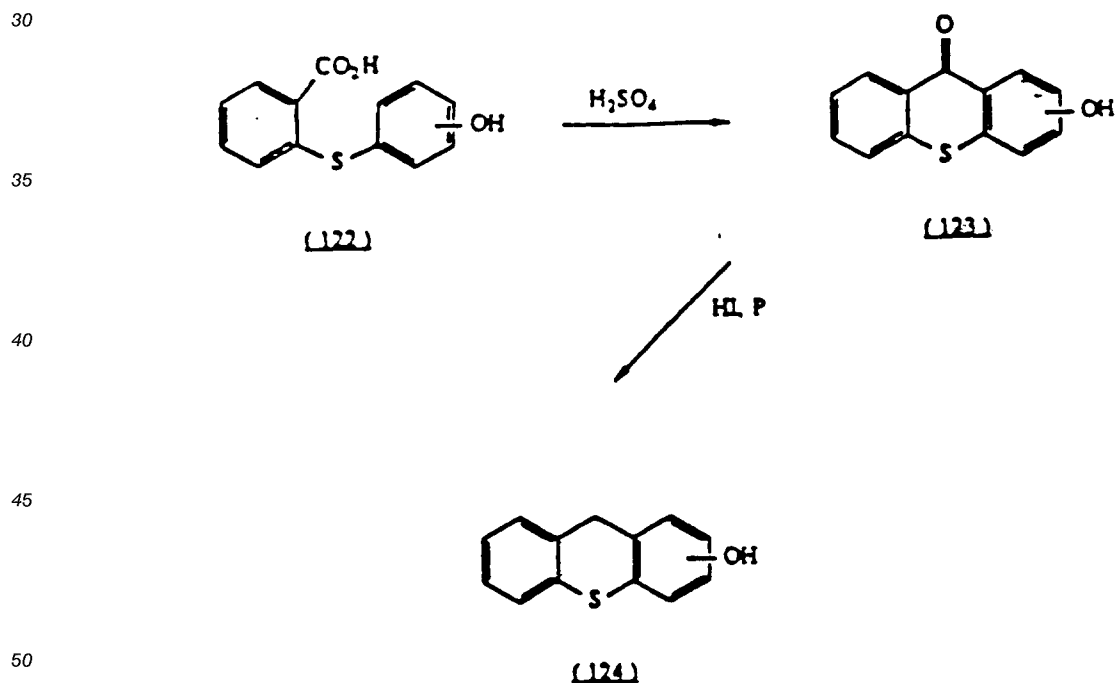
Scheme 56
