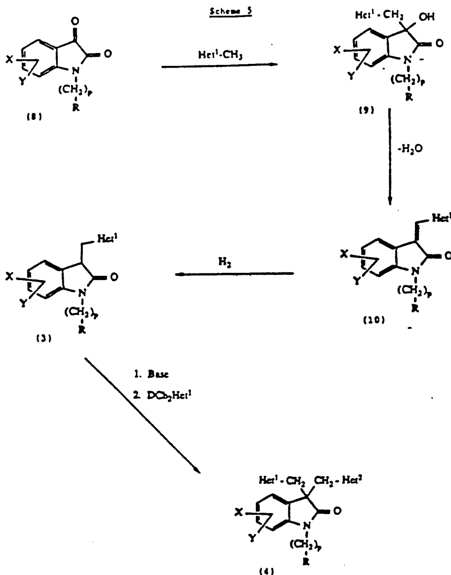
Scheme 5
