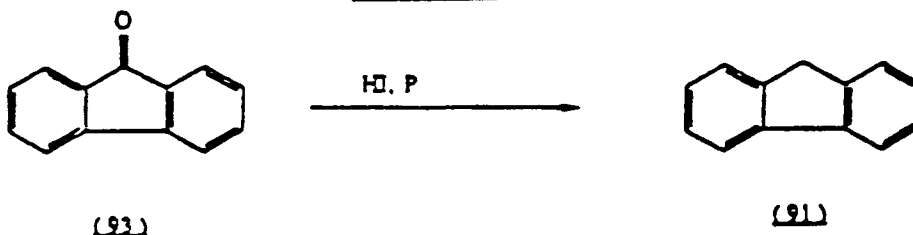
Scheme 42
