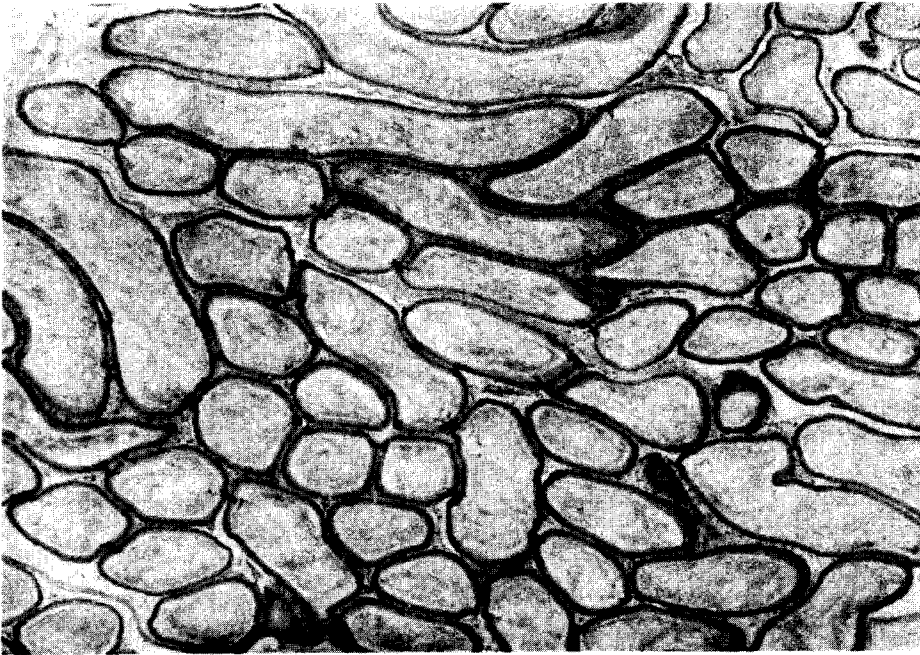
CONTROL EPIDIDYMIS
