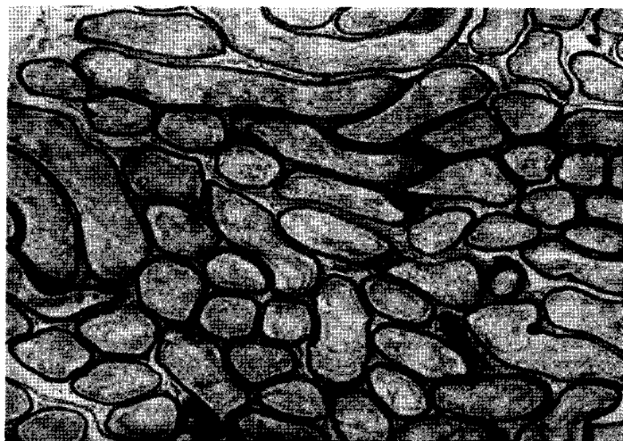
CONTROL EPIDIDYMIS
