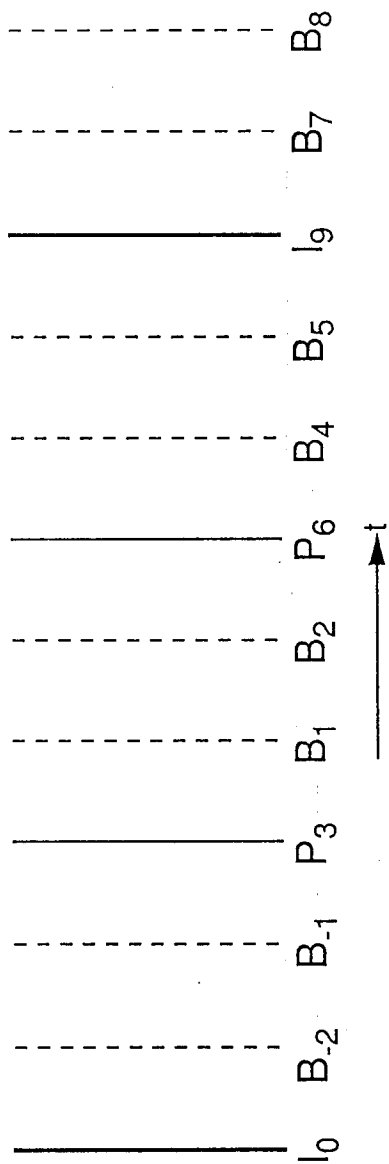
Frame Processing Order at Decoder Fig. 18
