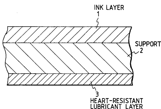
INK RIBBON
