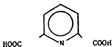
2,6-Pyridine Dicarboxylic Acid
