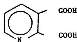
2,3-Pyridine Dicarboxylic Acid
