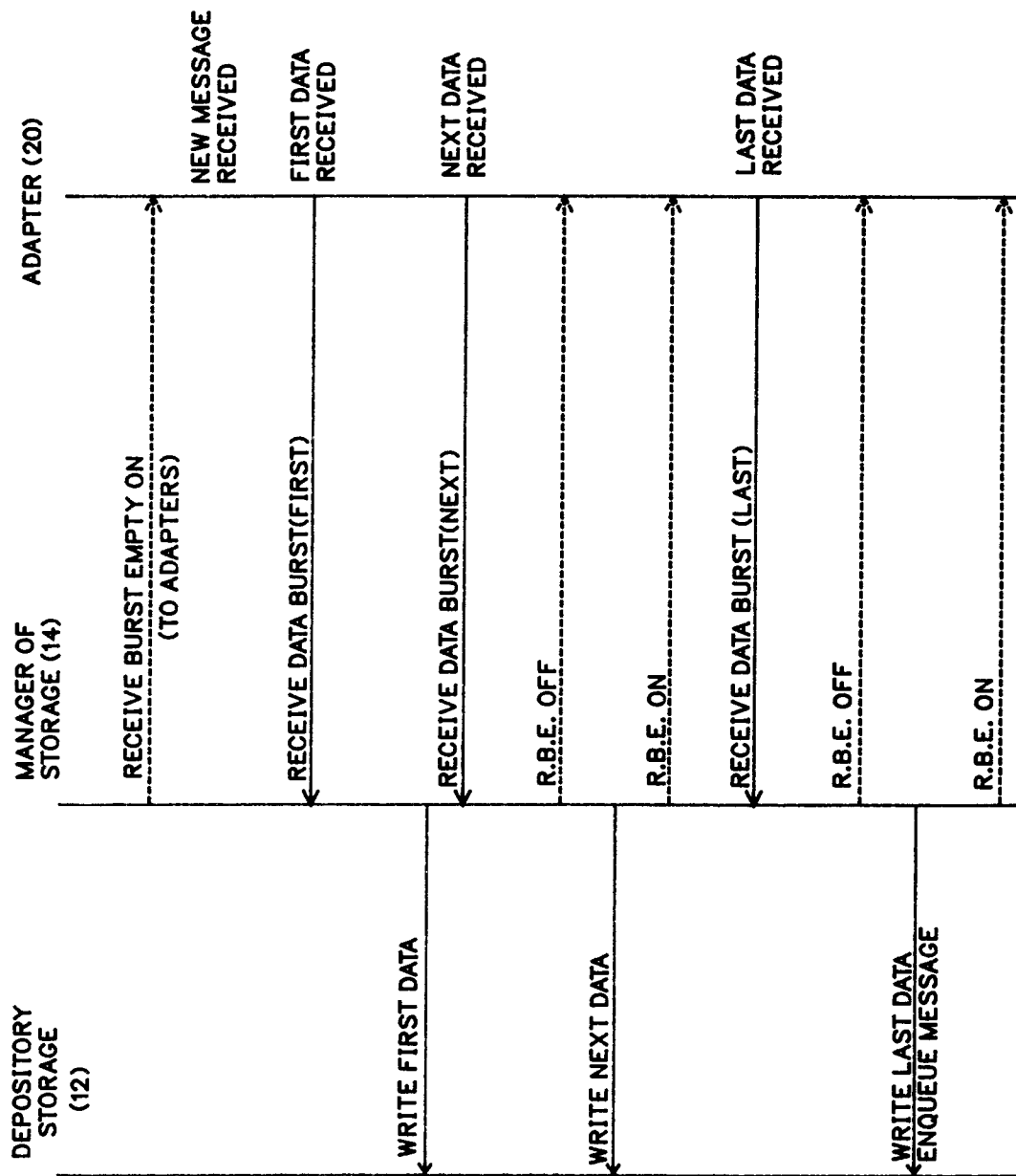
AN EXAMPLE OF A MESSAGE RECEIVED IN THE SHARED MEMORY SUBSYSTEM FIG. 5C
