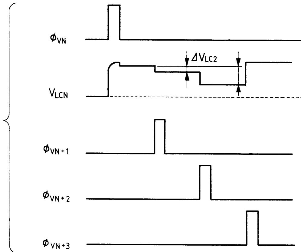
FIG. 6 PRIOR ART
