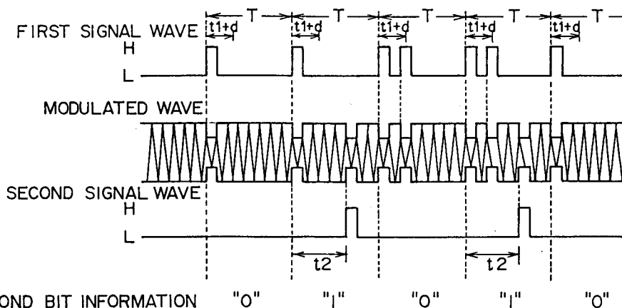
FIG. 8(a) FIRST BIT INFORMATION "0" "0" "1" "1" "0"
