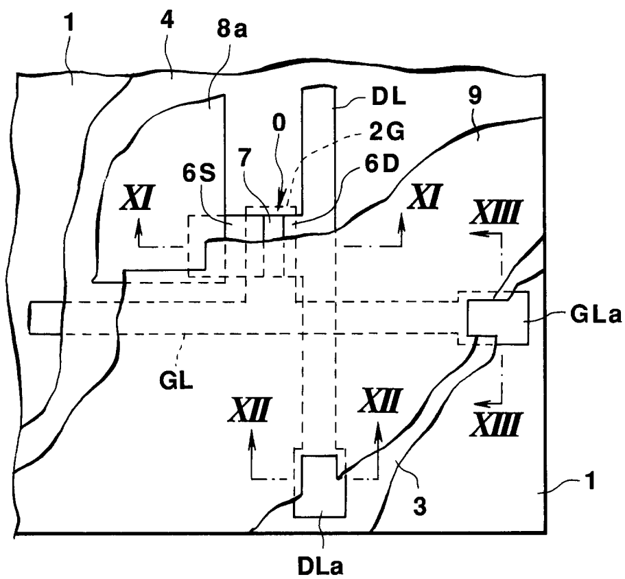
FIG. 10 (PRIOR ART)
