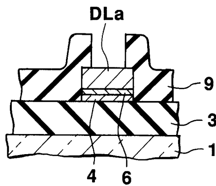
FIG. 12 (PRIOR ART)
