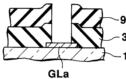
FIG. 13 (PRIOR ART)
