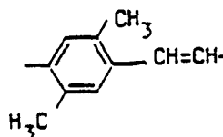
2,5-dimethyl-para-phenylene vinylene (PDMPV)
