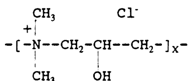
Principal repeating unit of Resin 6
