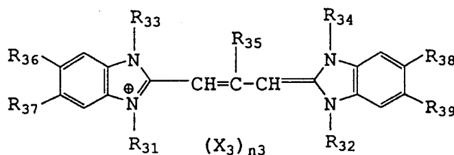
Formula III
