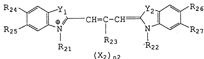
Formula II
