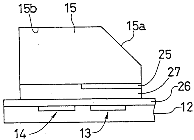
FIG. 5 PRIOR ART
