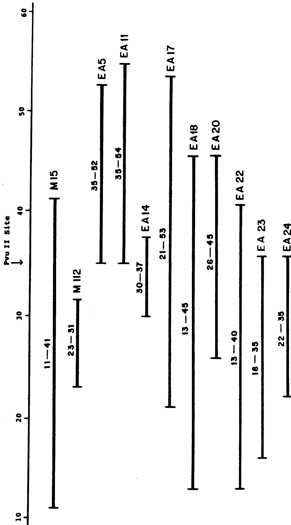
FIG. 5A Enzyme-Acceptor Mutants ( \alpha -Region) of \beta -galactosidase
