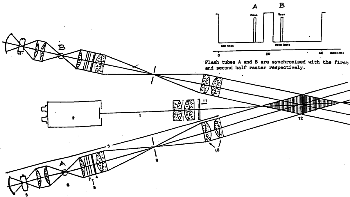
Fig. 1: Diagram of the projection and registration part of the keratometer according to the invention.
