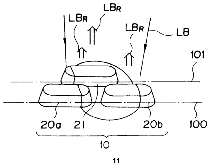
FIG. 1C PRIOR ART
