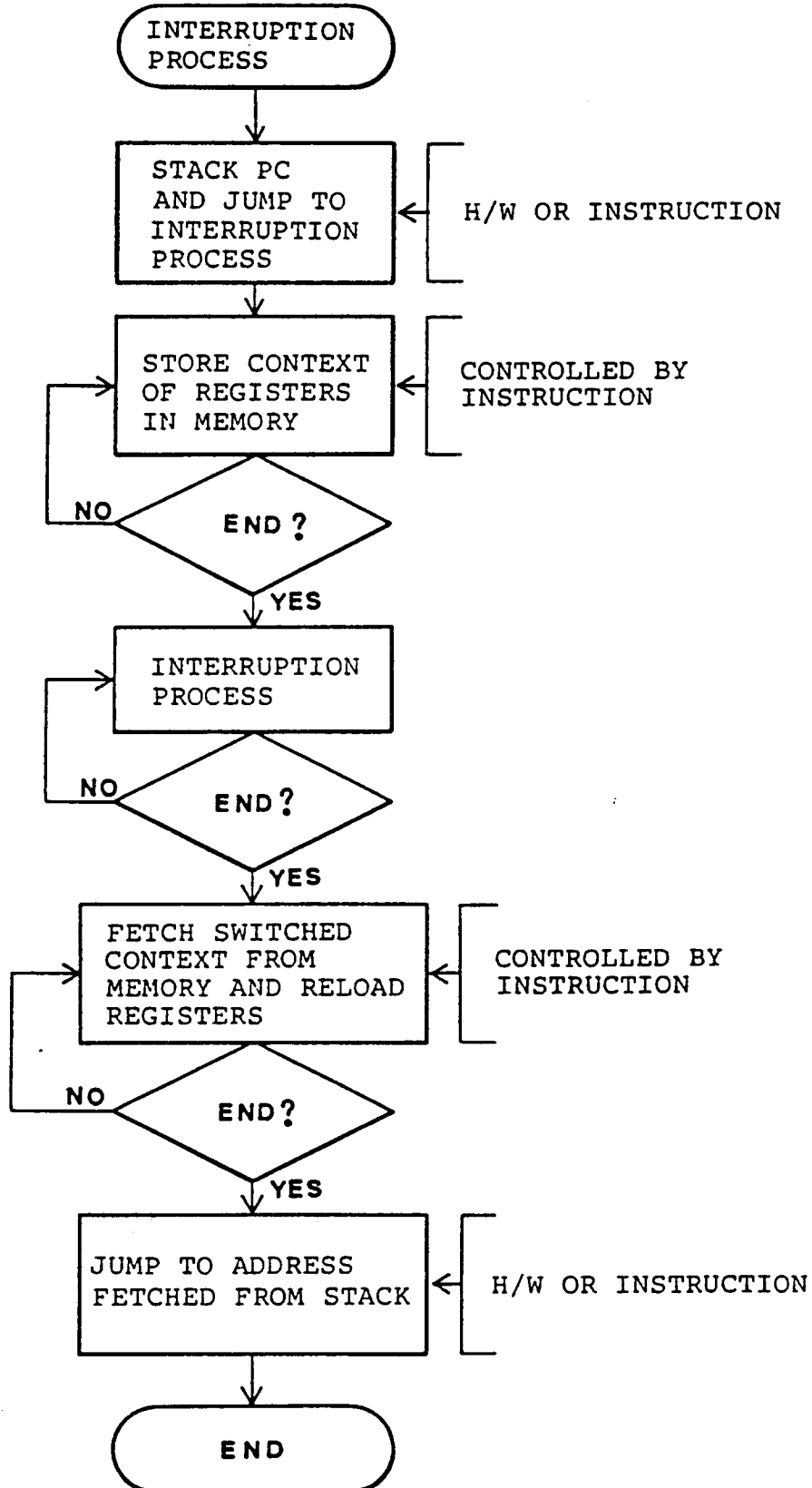
Fig. 14 (PRIOR ART)
