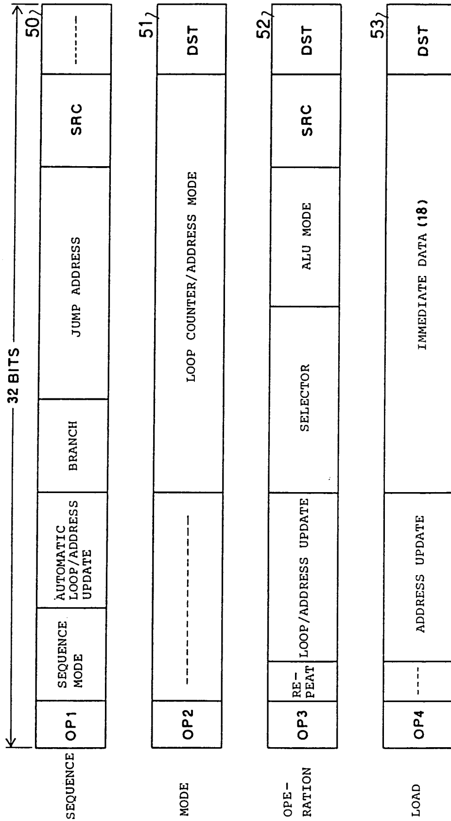
Fig. 3 (PRIOR ART)
