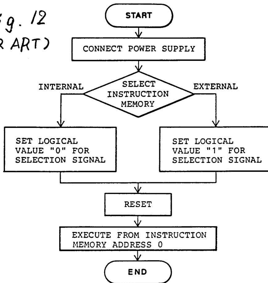
Fig. 23 (PRIOR ART)
