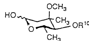
Compounds (7), (8) and (21) - (26)
