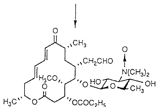
Compound (3)
