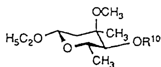
Compounds (5), (6) and (15) - (20)
