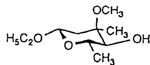
Compound (4)
