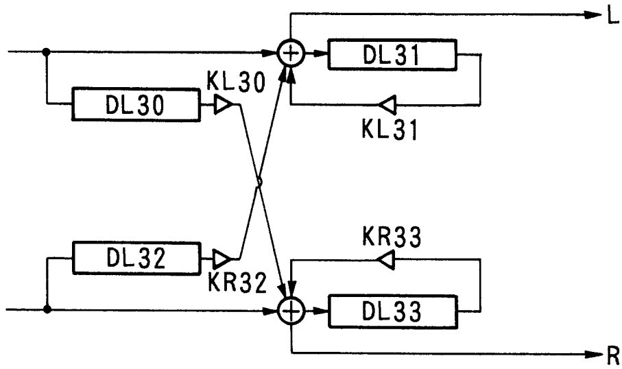
FIG.3(A) (DETAILED CONFIGURATION OF CROSS-TALK CANCELER 2)
