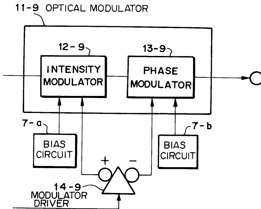
OPTICAL TRANSMITTER 100-9
