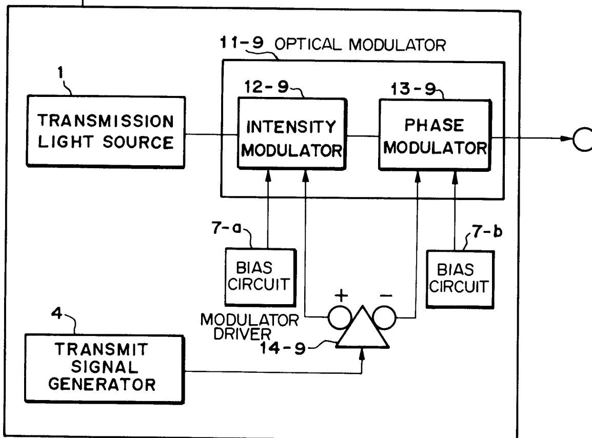
OPTICAL TRANSMITTER 100-9
