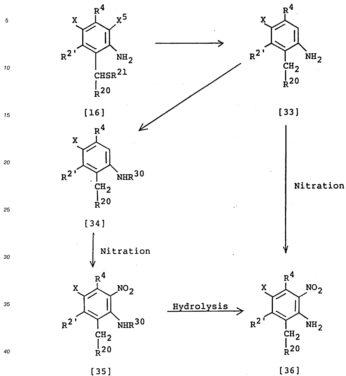
[Reaction scheme-X]
