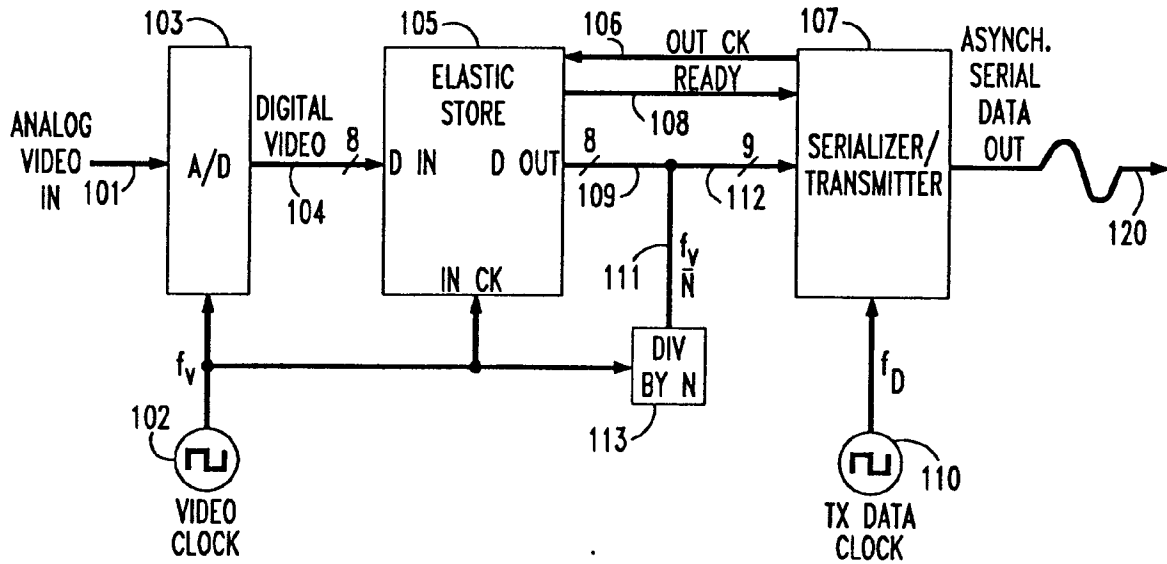
FIG. 1 TRANSMITTER UNIT 100
