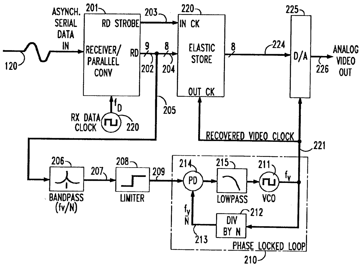
FIG. 2 RECEIVER UNIT 200
