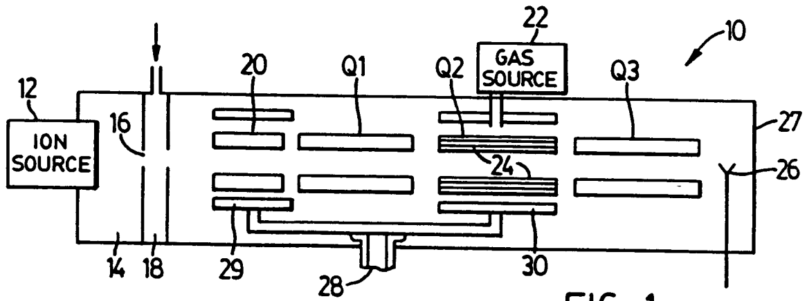
FIG. 1 (PRIOR ART)
