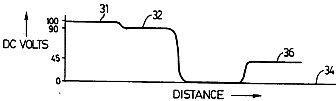
FIG. 2 (PRIOR ART)
