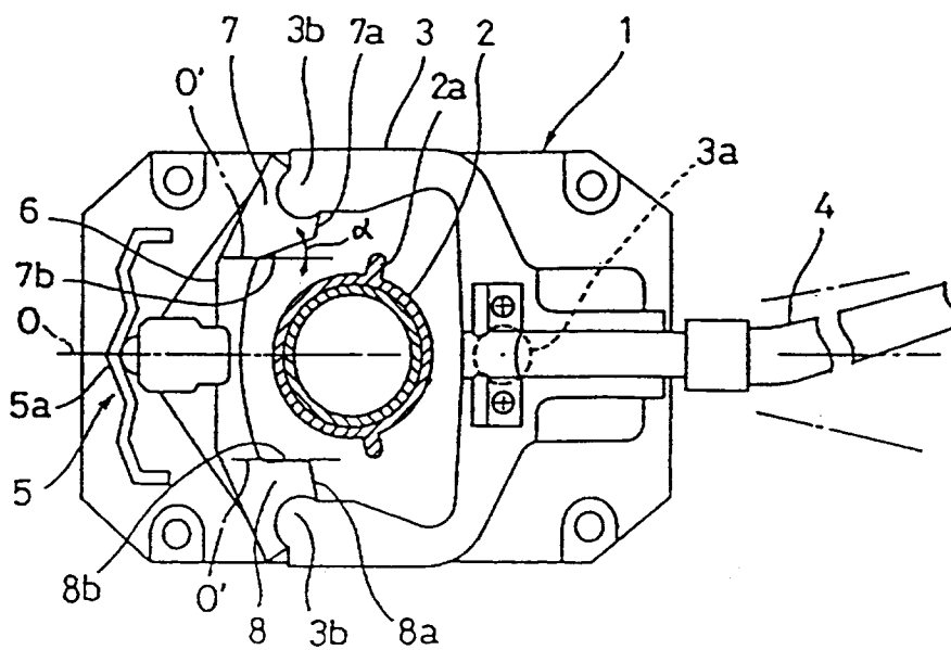
FIG. 10 PRIOR ART
