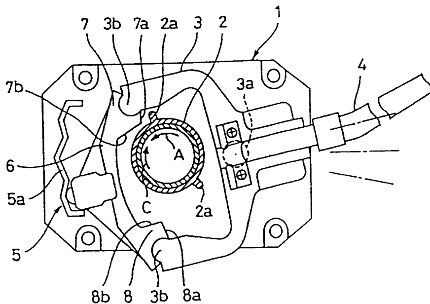
FIG. 11 PRIOR ART
