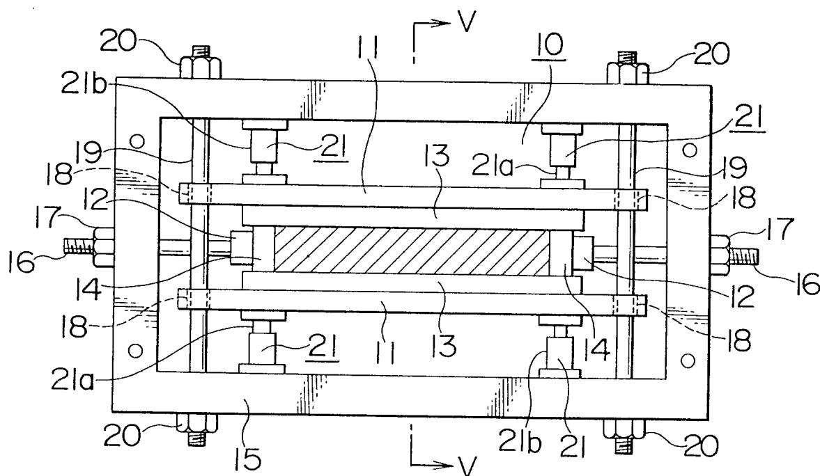
FIG. 1 PRIOR ART
