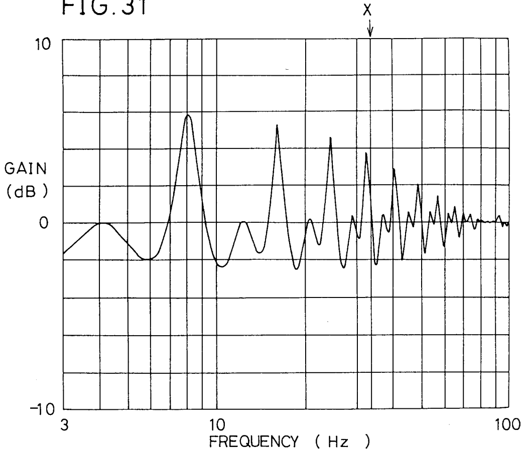
FIG. BODE DIDAGRAM OF SERVORESPONCE
