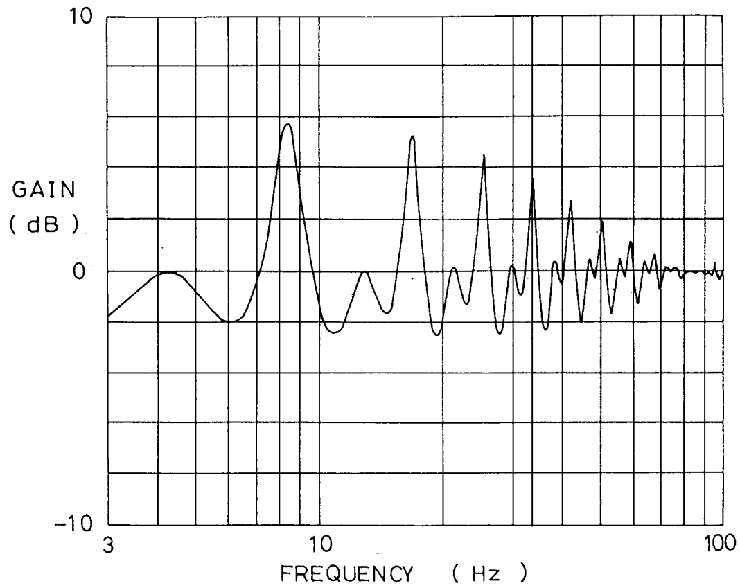
FIG. BODE DIDAGRAM OF A.I. SERVORESPONCE
