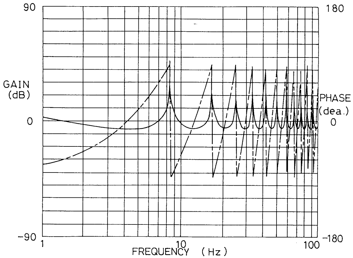
FIG. BODE DIDAGRAM OF SERVO RESPONCE
