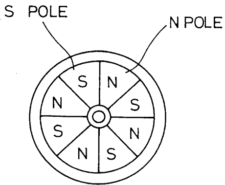
ROTOR MAGNET
