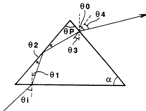
FIG.5 (PRIOR ART)
