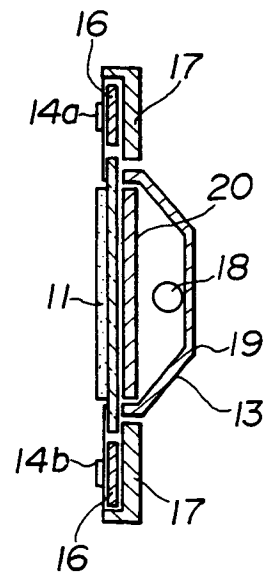
FIG.8B (PRIOR ART)
