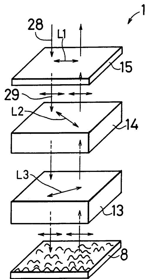
Fig. 6 (2) (TRANSMITTING REFLECTED LIGHT)
