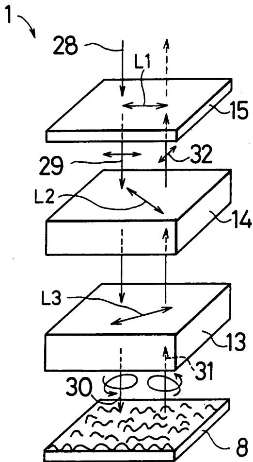
Fig. 6 (1) (SHIELDING REFLECTED LIGHT)
