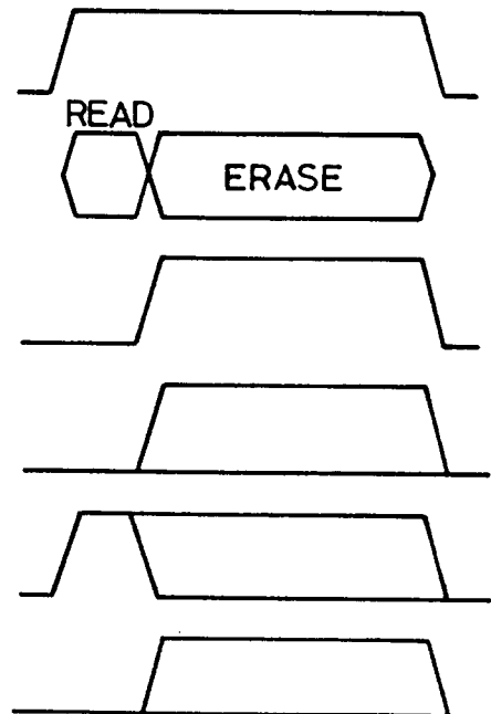
FIG. 8A ALL SELECT SIGNAL AS
