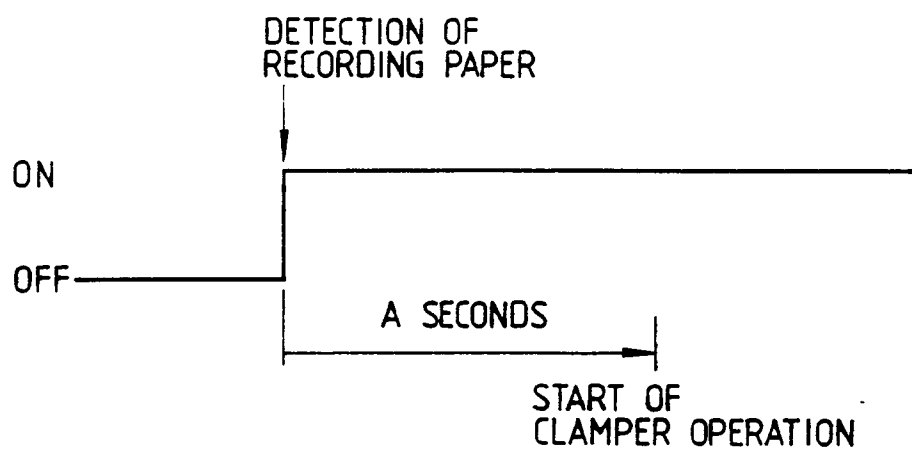
FIG. 5 PRIOR ART
