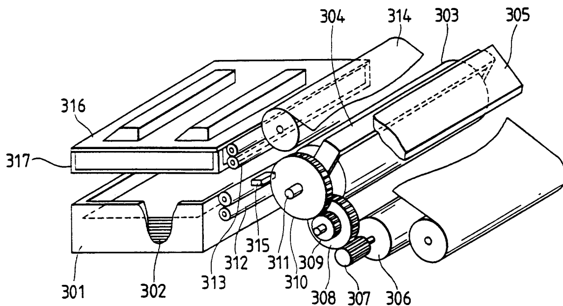
FIG. 14 PRIOR ART
