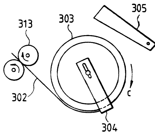
FIG. 18 PRIOR ART
