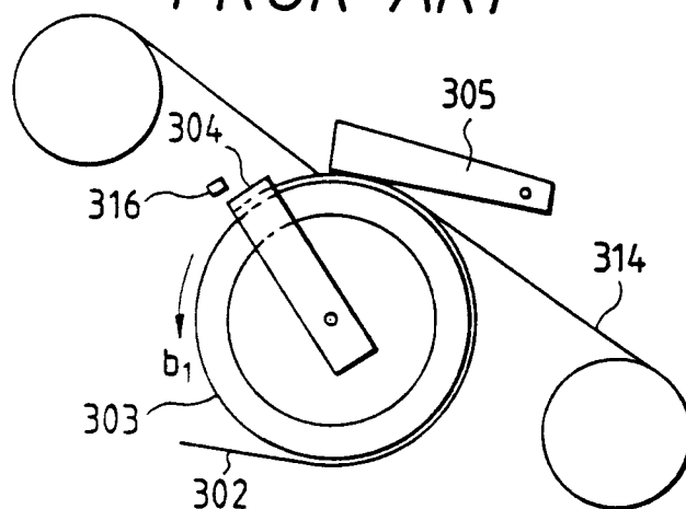
FIG. 18 PRIOR ART
