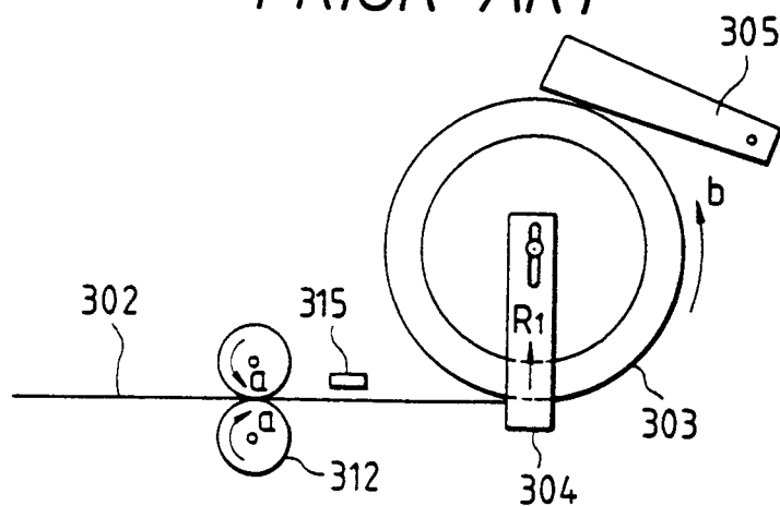
FIG. 17 PRIOR ART
