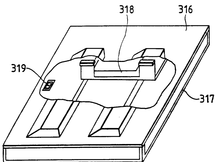
FIG. 15 PRIOR ART
