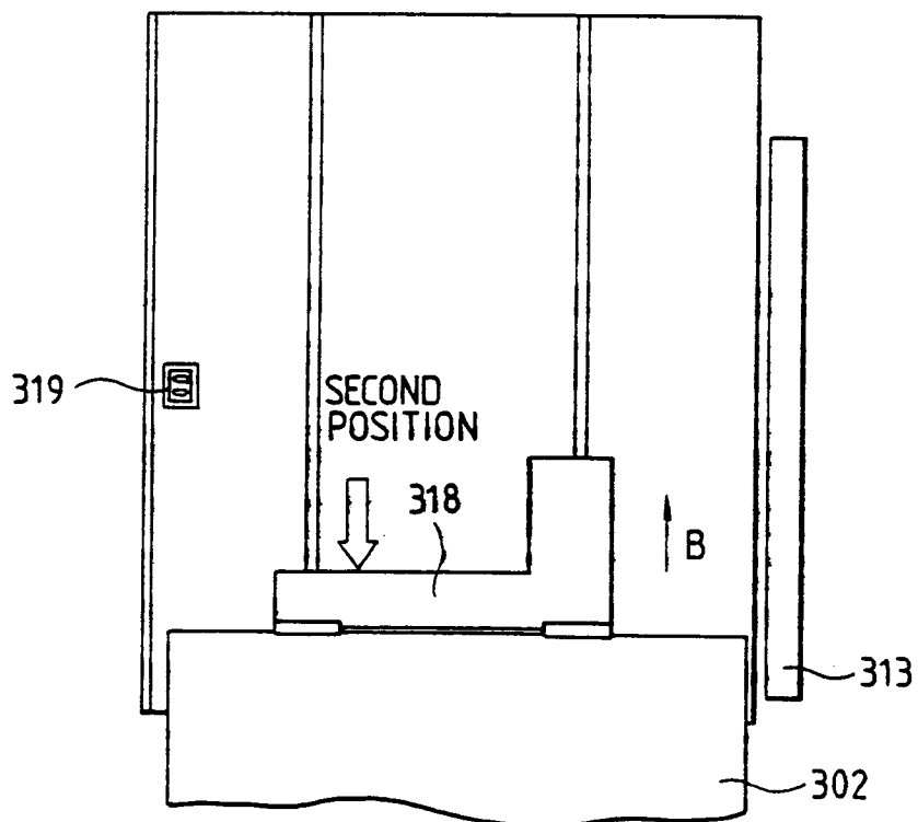
FIG. 22 PRIOR ART
