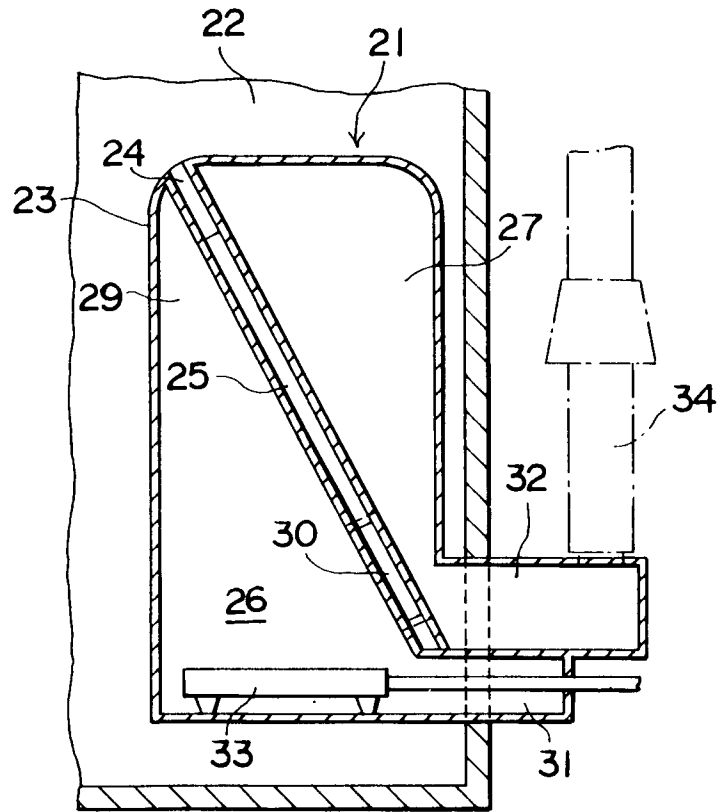
FIG. 9 PRIOR ART
