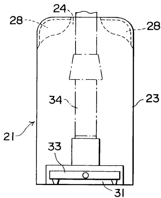
FIG. 10 PRIOR ART
