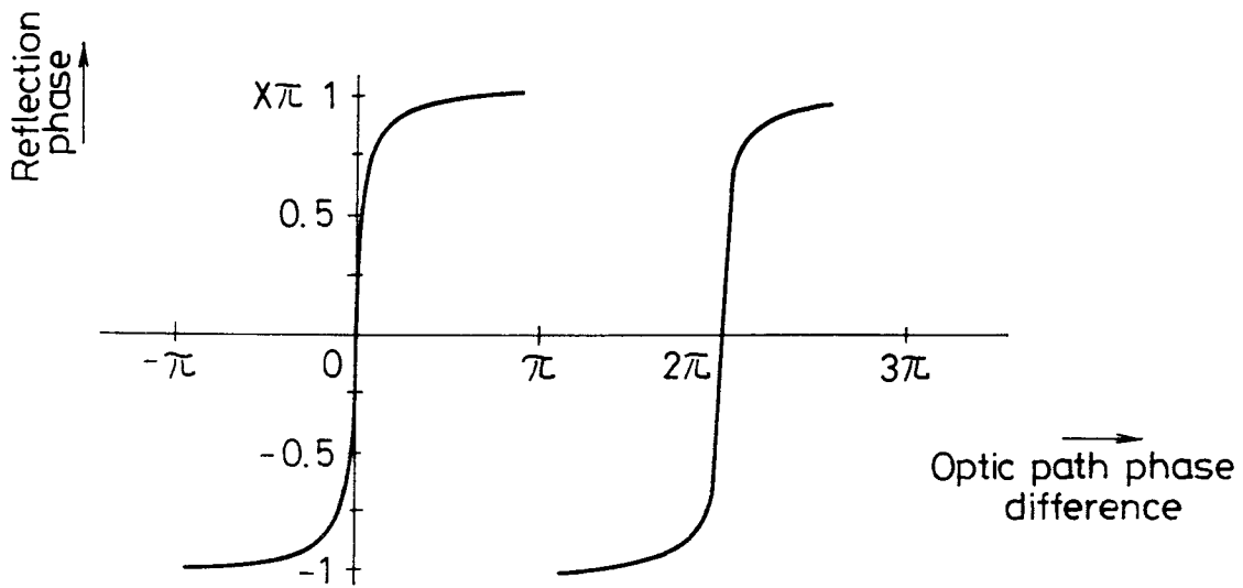
Graph of phase of reflectance r
