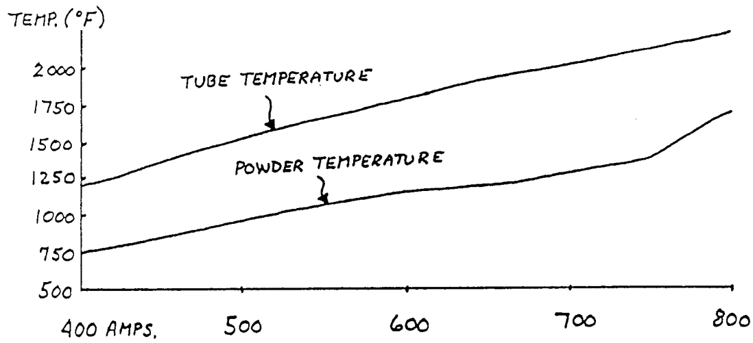
FIG. 3 TUBE CURRENT
