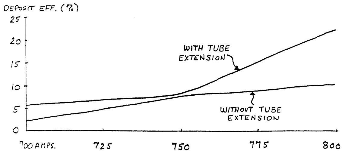
FIG. 5 TUBE CURRENT
