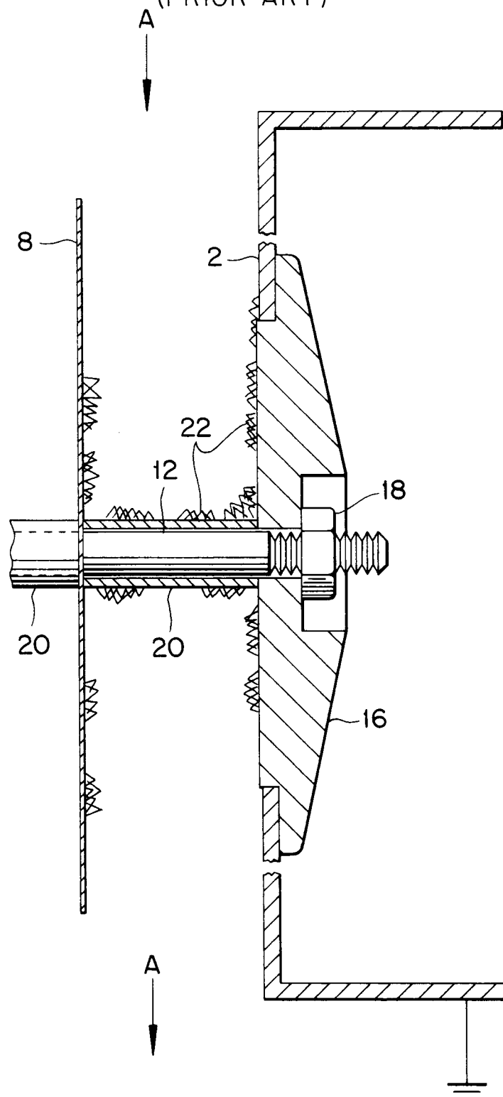
FIG. 2 (PRIOR ART)
