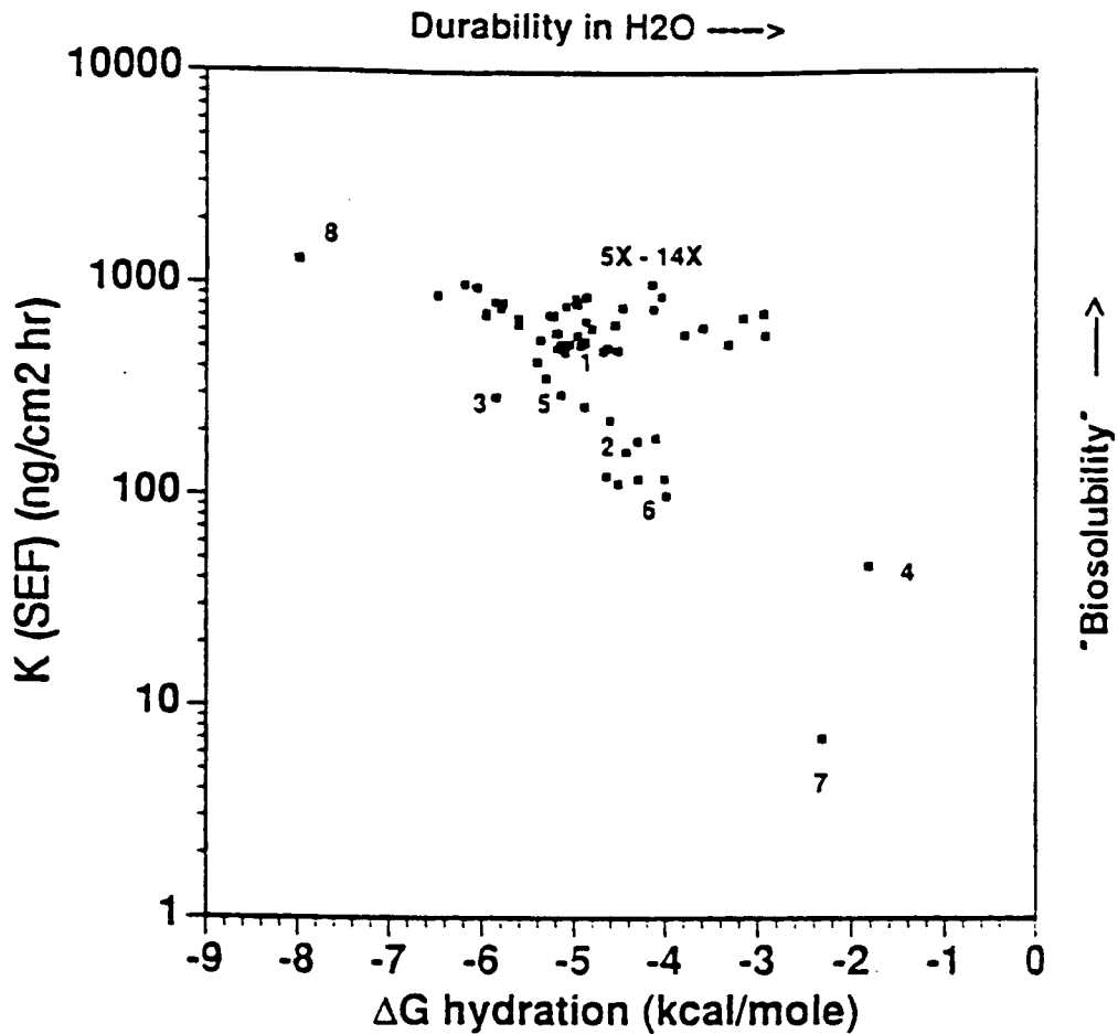
Figure 2. Correlation between dissolution rate constant in simulated extracellular fluid (SEF) and free energy of hydration for the glass comprising fibers developed in this study. Plot assumes only those reactions involving hydration of the glass are significant. Values for fiber compositions 1 through 8 in Tables 3 and 5 are indicated together with those for the experimental 5X through 14X series..
