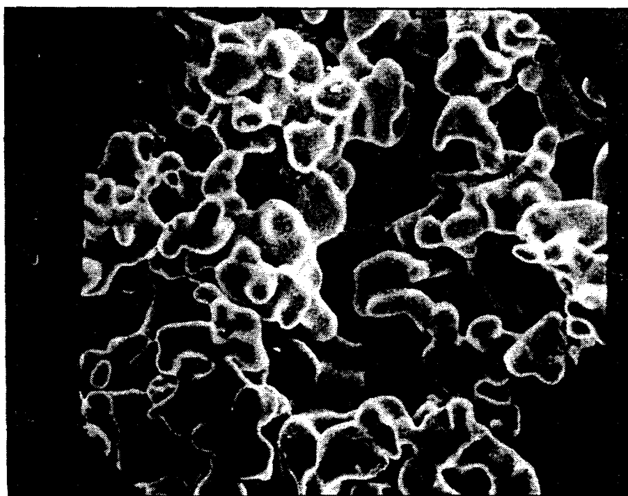
Fig. 3 SINTERED Cu/Ni ON LiFeO 2 -1,000X
