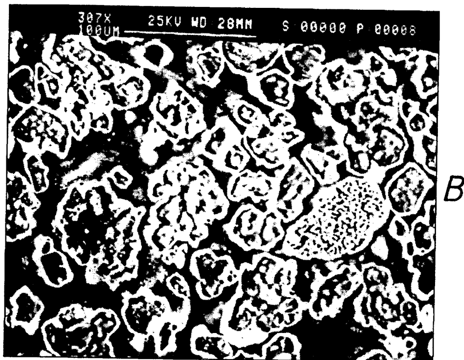
Fig . 8 MICROGRAPHS OF METAL COATED ANODES (SHOW IMPROVEMENT OF ENGINEERED METAL COATED CERAMIC MICROSTRUCTURE:-METALLIC PHASE APPEARS LIGHTER) A). AS-RECEIVED ANODE PLAQUE XXII-1 FROM BATCH 3 B). AS-RECEIVED PLAQUE LXXVIII-8 FROM BATCH 8
