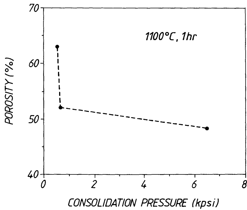
EFFECT OF SINTERING CONSOLIDATION PRESSURE ON THE POROSITY OF LIFE O 2 ANODES
