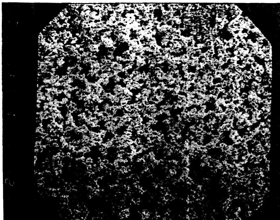
Fig. 2 SINTERED Cu/Ni ON LiFeO 2 -1,00X
