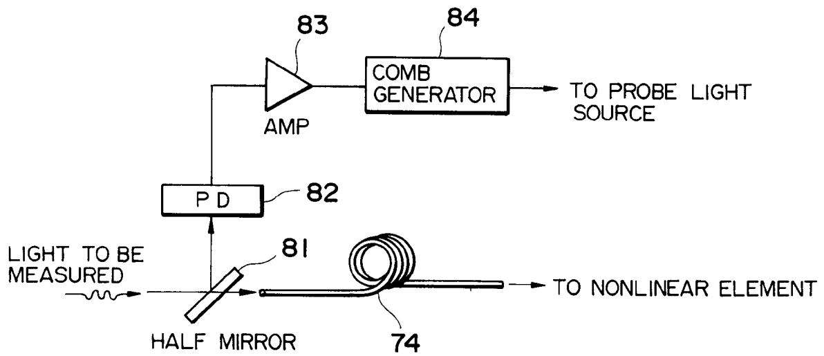
EXAMPLE OF MEASURED LIGHT ARRIVAL DETECTOR
