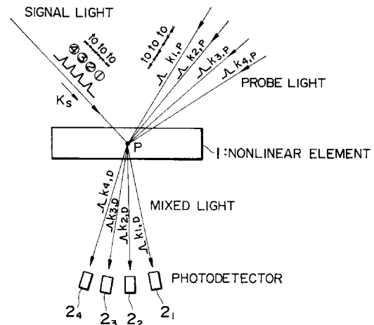
ILLUSTRATION OF BASIC OPERATION IN OPTICAL SERIAL-PARALLEL CONVERTER
