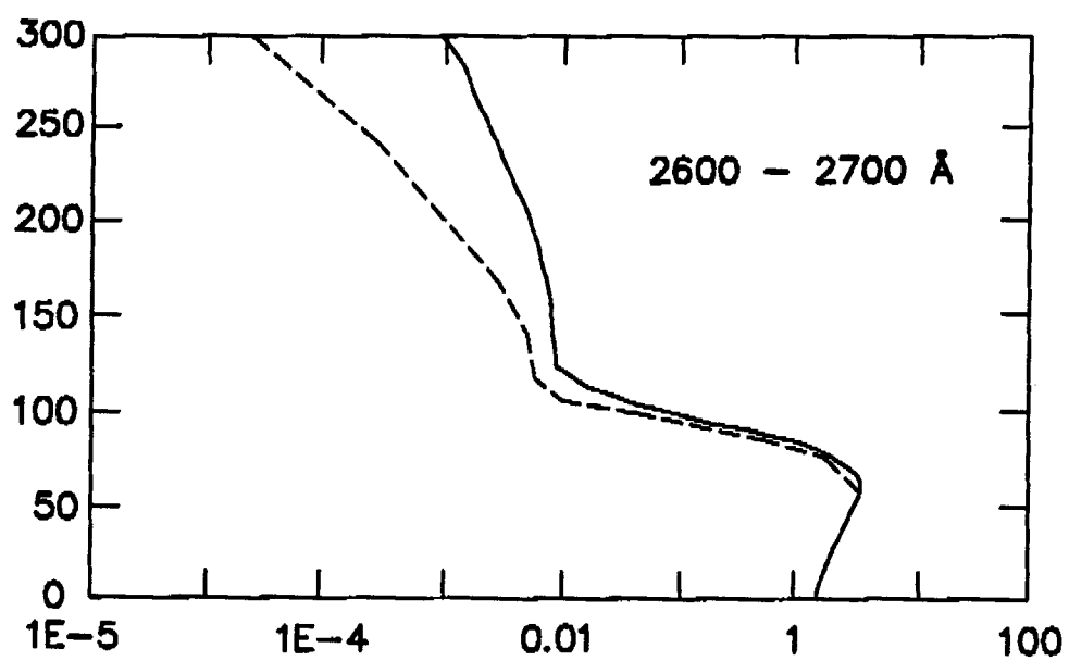
Limb Intensity Profile (maximum noon brightness)
