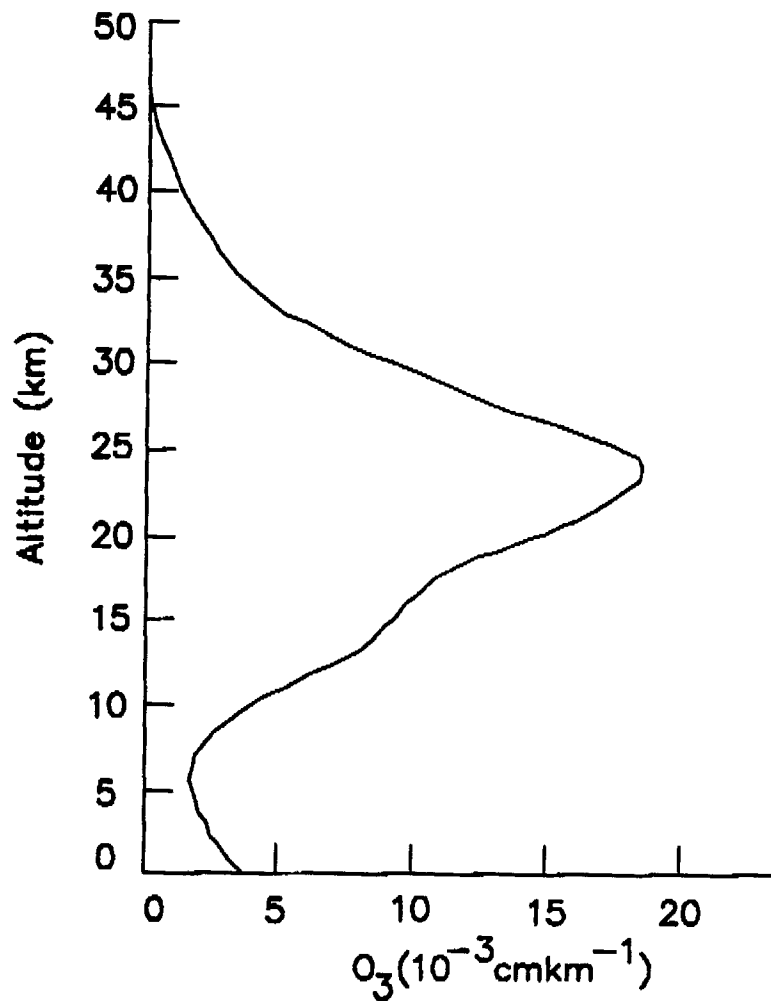
Altitude Distribution of Ozone
