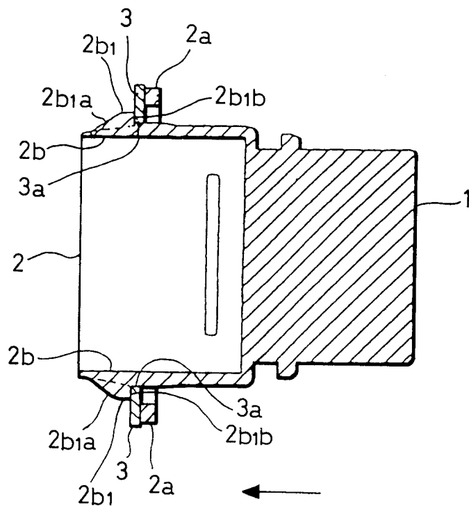
FIG. 10 (RELATED ART)
