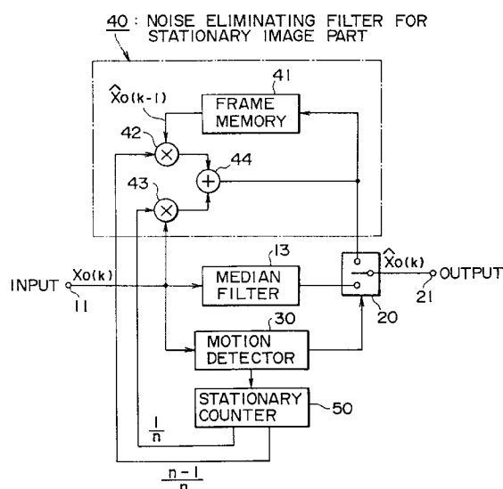
NOISE ELIMINATING CIRCUIT 10
