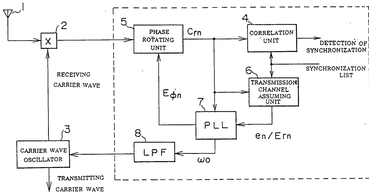
BLOCK DIAGRAM OF A RECEIVER OF THE INVENTION
