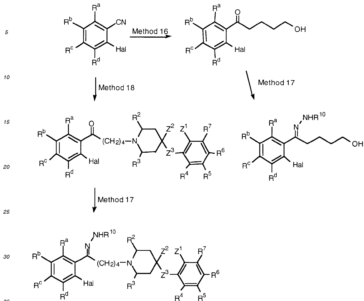
Scheme 6
