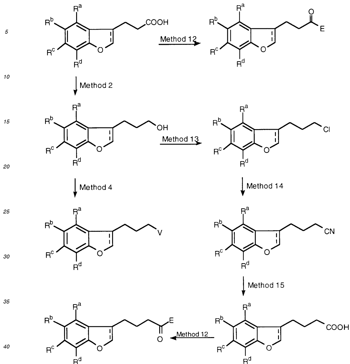
Scheme 5
