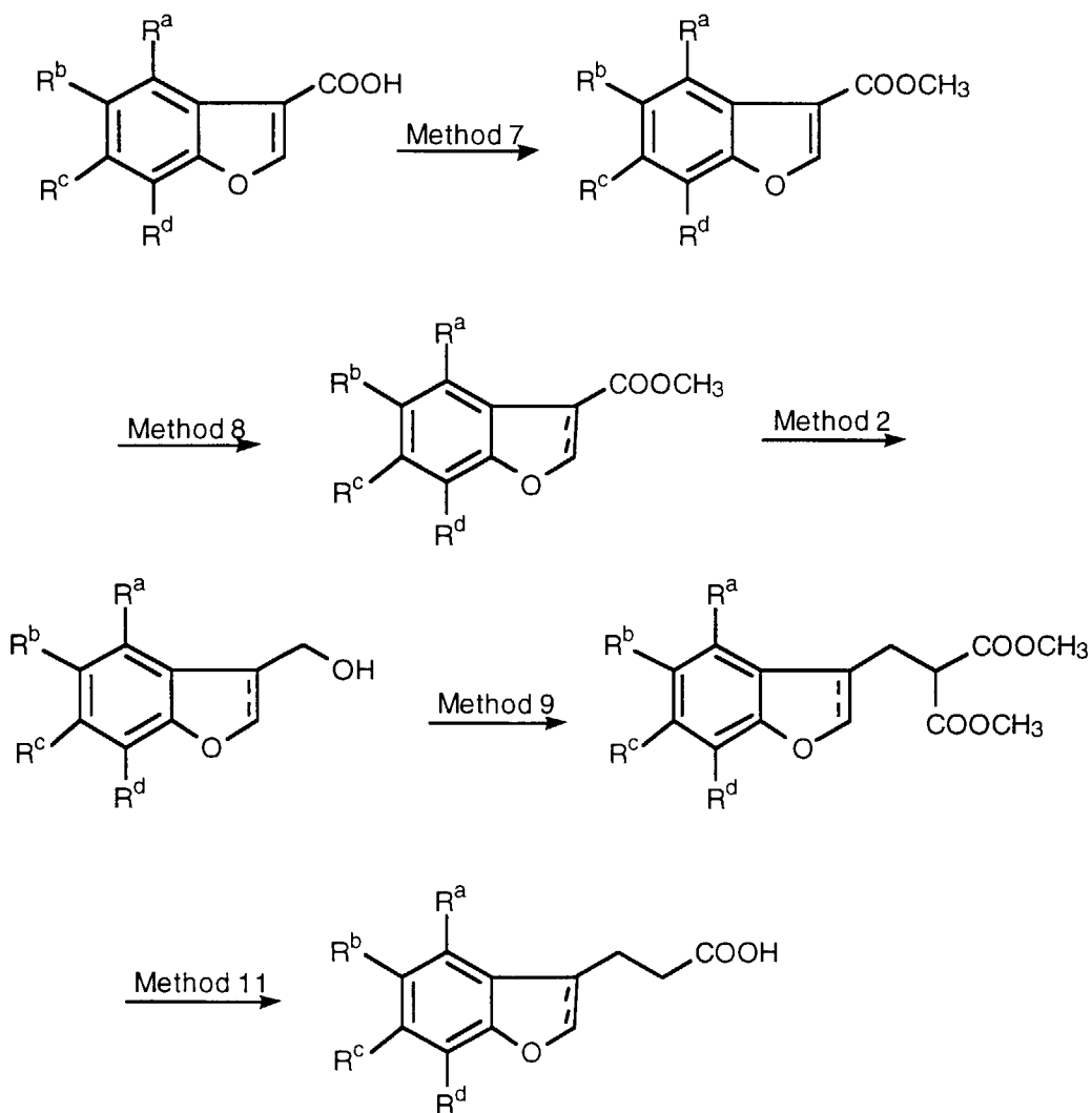
Scheme 4
