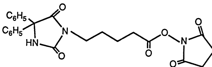
CBDH N-hydroxysuccinimide ester (PTN Linker Intermediate)
