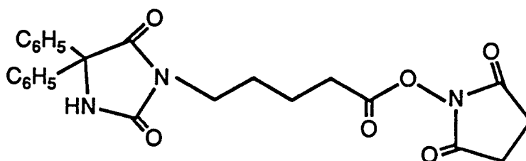
CBDH N-hydroxysuccinimide ester (PTN Linker Intermediate)
