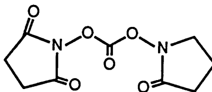
Disuccinimidyl carbonate (DSC)
