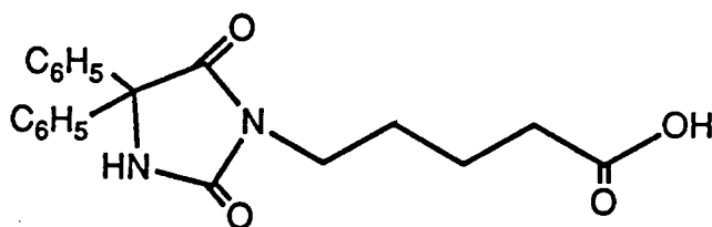
Carboxy butyl diphenylhydantoin (CBDH)
