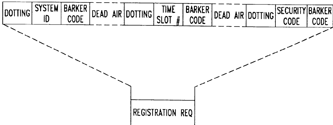
FIG. 6 REGISTRATION REQUEST FRAME
