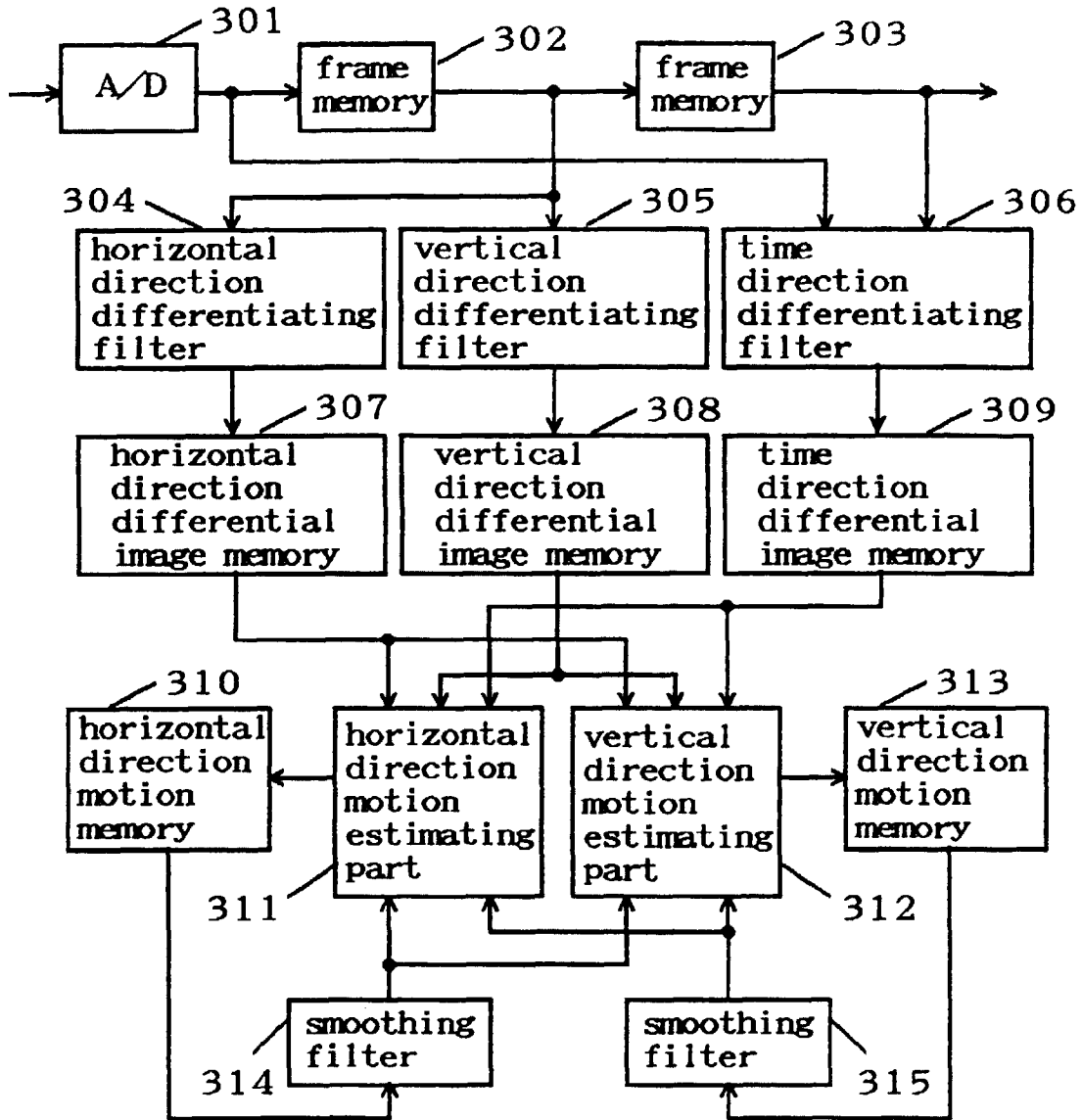
Fig. 1 (PRIOR ART)
