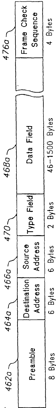
Ethernet Frame Format
