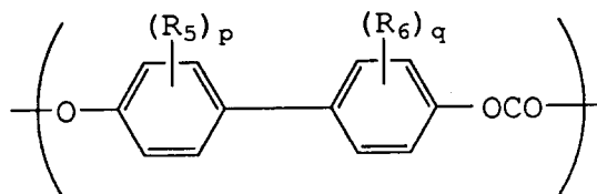
Formula (B 2 )
