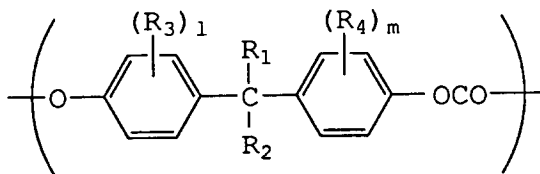
Formula (B 1 )
