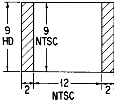
DISPLAY OF NTSC IMAGE BY HDTV MONITOR
